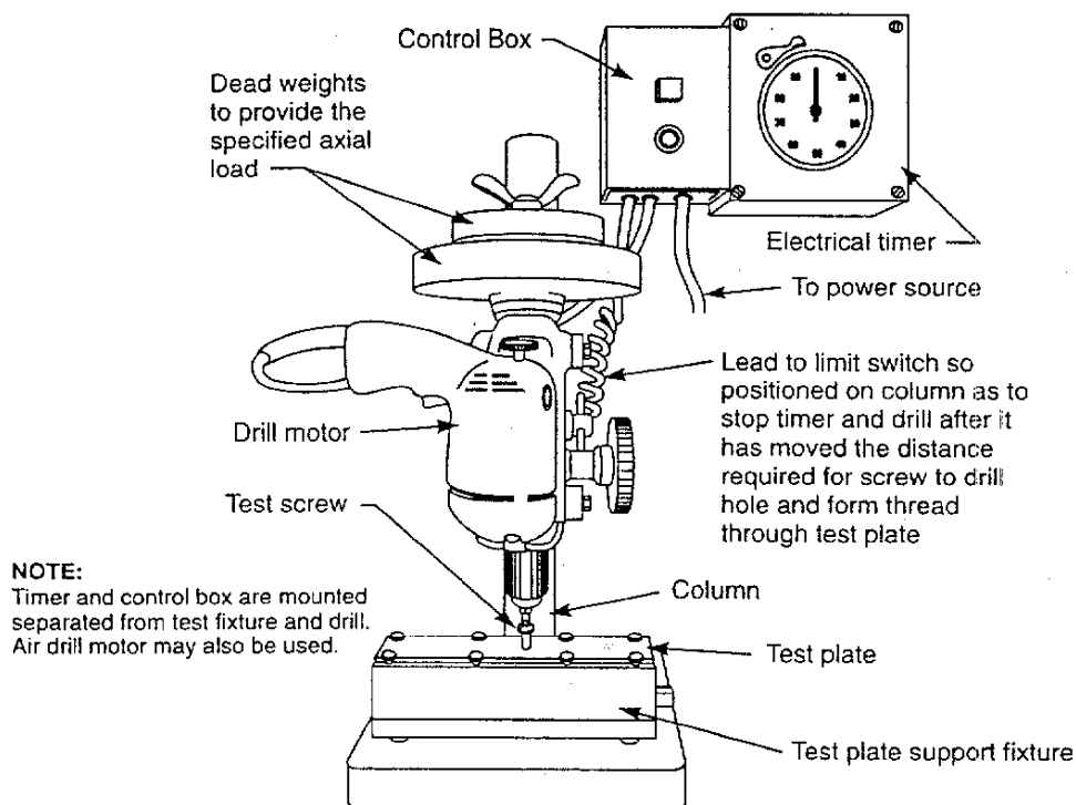
Fig. 4 Typical Drill-Drive Test Fixture
