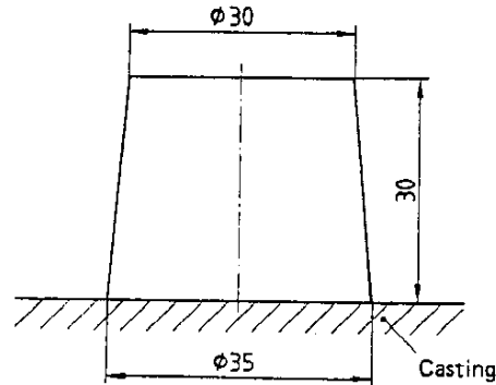
Figure 3. Cast-on sample for testing Brinell hardness
