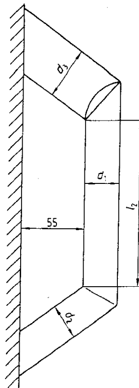
Figure 2. Type H cast-on test piece
