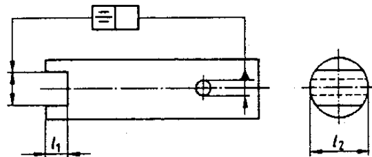
c) Datum: longer feature ( l_2 )
