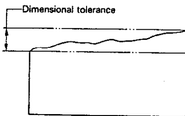
Figure B.3 — Parallelism deviation equal to the numerical value of the size tolerance
