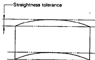
Figure B.4 — Parallelism deviation equal to the numerical value of the straightness tolerance
