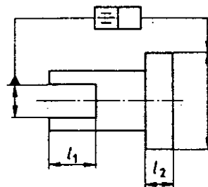
b) Datum: longer feature ( l_1 )
