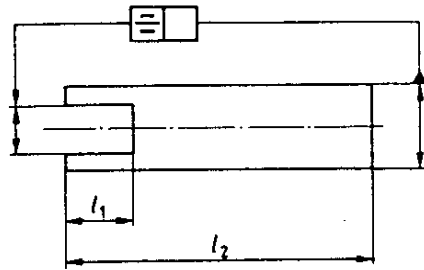
a) Datum: longer feature ( l_2 )
